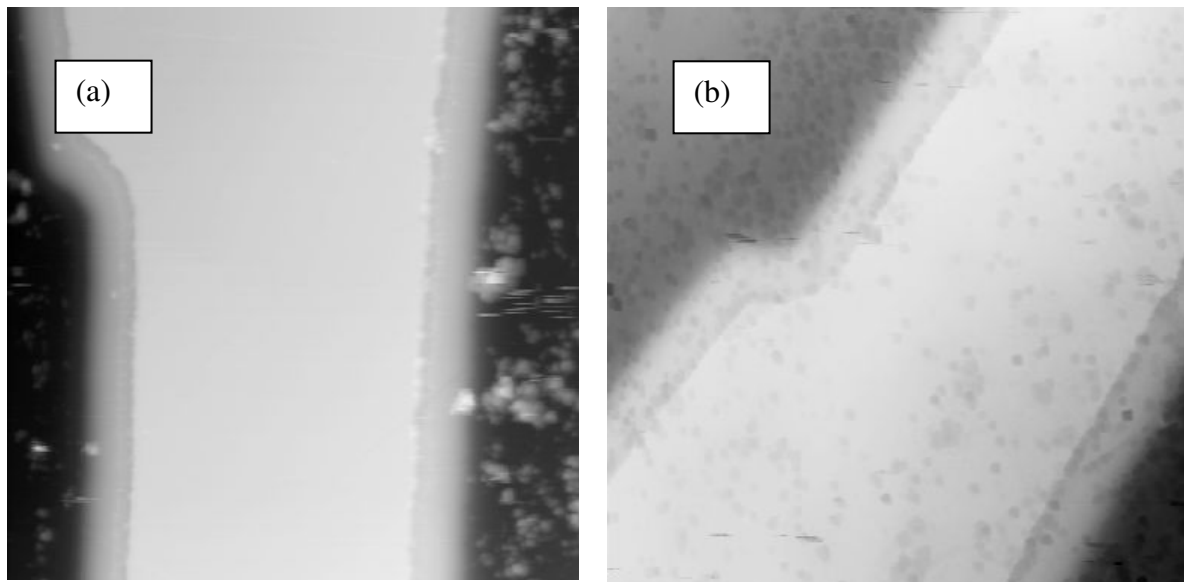
Figure 3: AFM images (32 \times 32) \mu\text{m}^2 of (a) silicon substrate with a z range of 500 nm and of (b) the corresponding region on the back of the diamond replica with a z range of 700 nm, with “treatment \frac{1}{4} \mu\text{m} ”.
