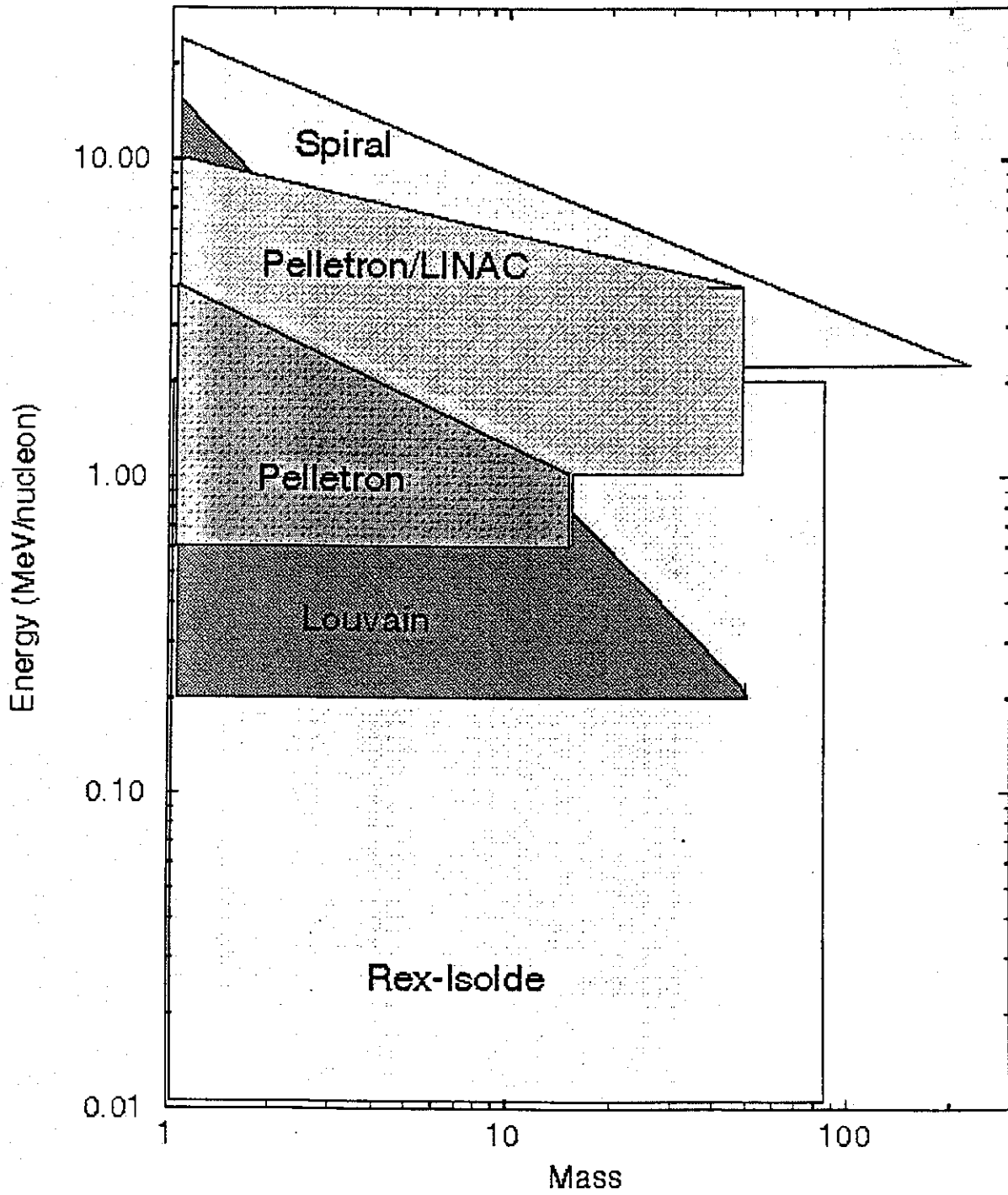
Figure 2: The regions in terms of mass and energy of operations of several RIB facilities.
