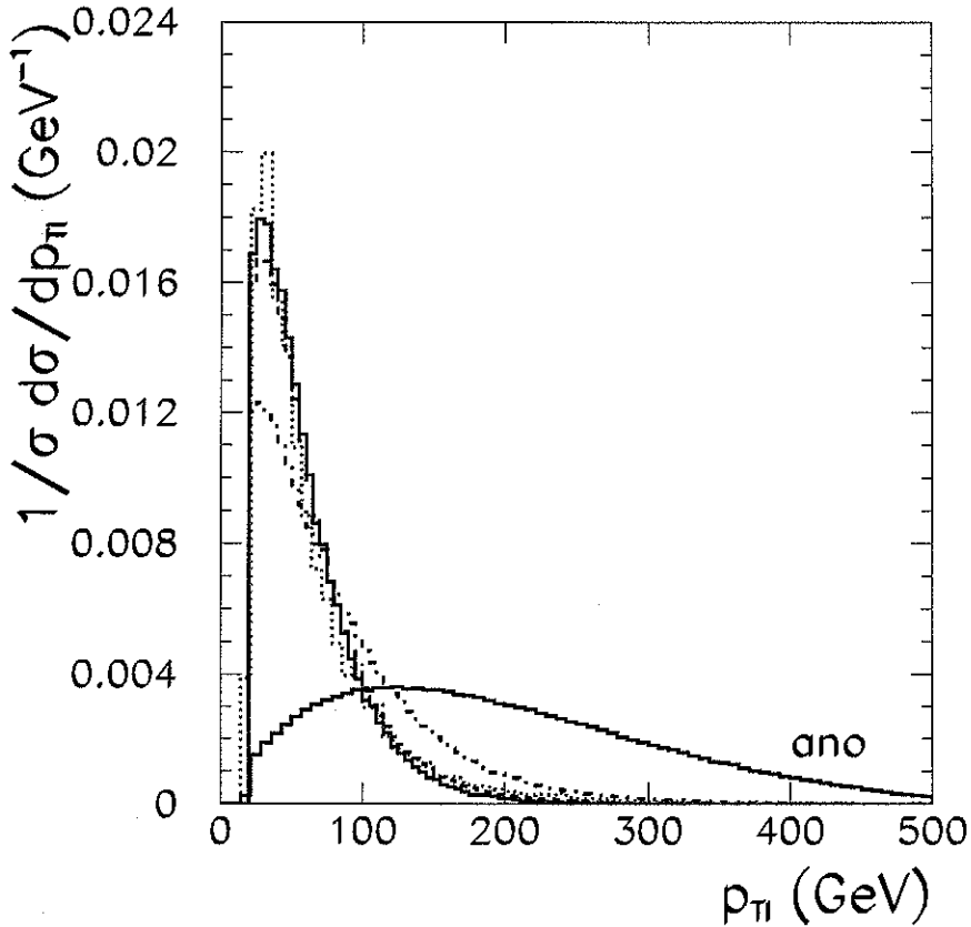
FIG. 1: Normalized distribution of the transverse momentum of the charge leptons for t\bar{t} (red solid line), t\bar{t}j (blue dashed line), t\bar{t}jj (black dot-dashed line), SM irreducible production (magenta dotted line), and anomalous W^+W^- contribution \sigma_{00} (blue solid line marked “ano”). We assumed m_h = 120 GeV and applied cuts (22)–(25) but for with a relaxed cut p_T^\ell > 20 GeV.
