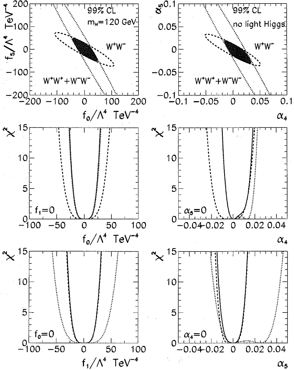
FIG. 8: Sensitivity bounds on the coefficients of the anomalous quartic gauge boson operators for the case with a light Higgs boson (left panels) and with no light Higgs boson (right panels). The upper panels show the 99% CL allowed regions for the different channels. The lower panels show the dependence of the \chi^2 function for the different channels assuming that only under that only one anomalous parameter is non-vanishing. The dashed (dotted) lines corresponds to pp \rightarrow jje^\pm\mu^\mp\nu\nu ( pp \rightarrow jje^\pm\mu^\pm\nu\nu ) while the combined analysis is indicated by the filled region and solid lines.
