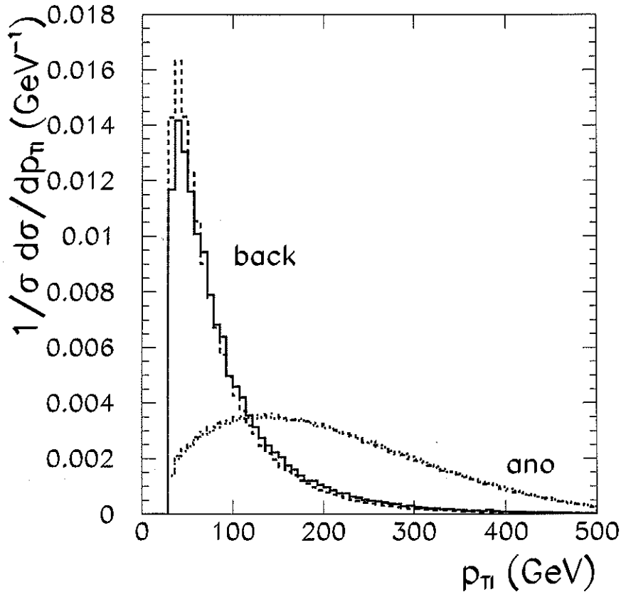
FIG. 5: Normalized lepton transverse momentum distribution for IRED++ background (solid line), IRED-- background (dashed line), W^+W^+ \sigma_{00} (dot-dashed line), and W^-W^- \sigma_{00} (dotted line). We assumed m_h = 120 GeV and applied cuts (22)–(25).
