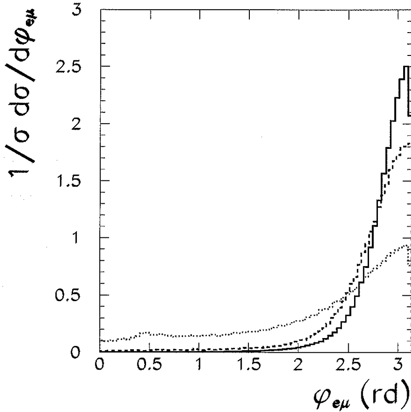
FIG. 3: Normalized distribution of the e\mu azimuthal angle difference for t\bar{t}j (dashed line), irreducible background (dotted line), and anomalous W^+W^- production (solid line). We assumed m_h = 120 GeV and applied cuts (22)–(27).
