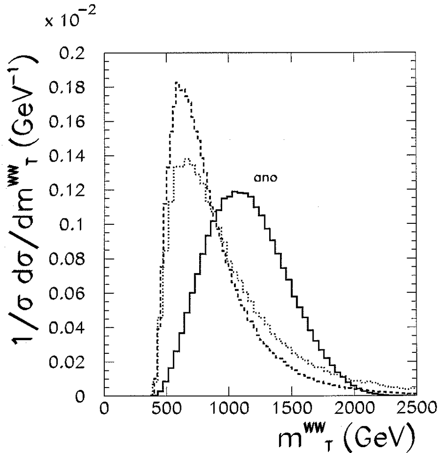
FIG. 4: Normalized distribution of M_T^{WW} for t\bar{t}j (dashed line), irreducible background (dotted line), and anomalous W^+W^- production (solid line). We assumed m_h = 120 GeV and applied cuts (22)–(28).
