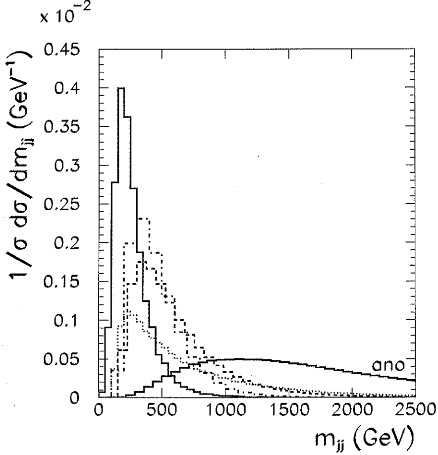
FIG. 2: Normalized jet-jet invariant mass distribution for t\bar{t} (red solid line), t\bar{t}j (blue dashed line), t\bar{t}jj (black dot-dashed line), SM irreducible production (magenta dotted line), and anomalous W^+W^- contribution \sigma_{00} (blue solid line marked “ano”). We assumed m_h = 120 GeV and applied cuts (22)–(25).
