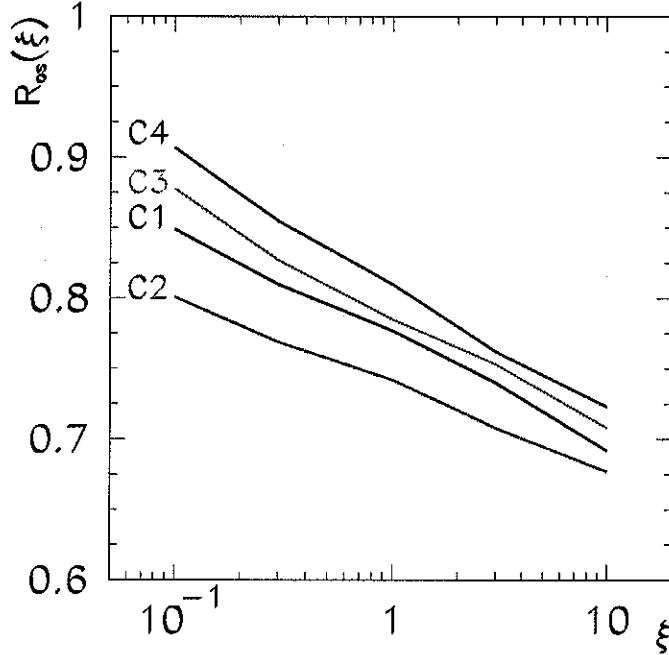
FIG. 7: The ratio R_{os} is shown as a function of \xi , where \mu_R = \xi\mu_R^0 for the four choices of renormalization and factorization scales given in the text.
