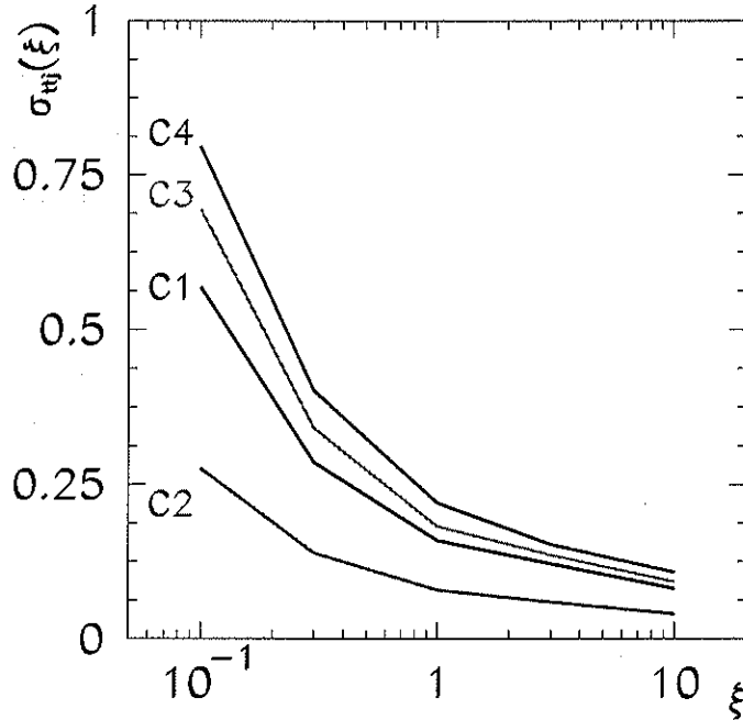
FIG. 6: Cross section for t\bar{t}j after cuts (22)–(28) as a function \xi , where \mu_R = \xi\mu_R^0 for the four choices of the factorization and renormalization scale defined in the text.
