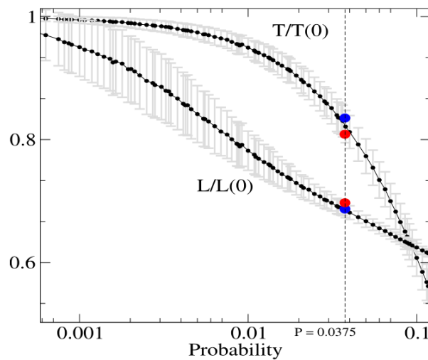
Fig. 4. Relative values of path length L/L(0) and transitivity T/T(0) as a function of the probability. The results for healthy and Alzheimer's networks are shown by blue and red dots, respectively. L(0) and T(0) correspond to the values of the path length and transitivity values for the regular network ( p = 0 ).
